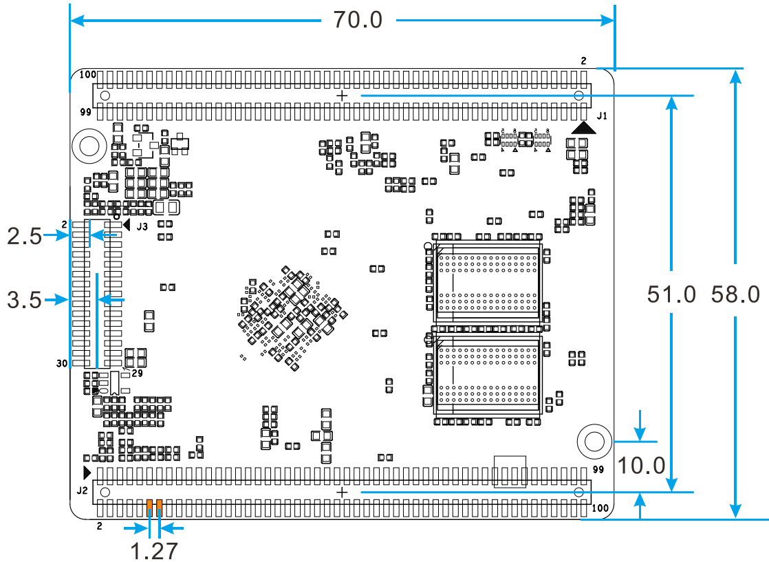
Figure 1. PCB Dimension
