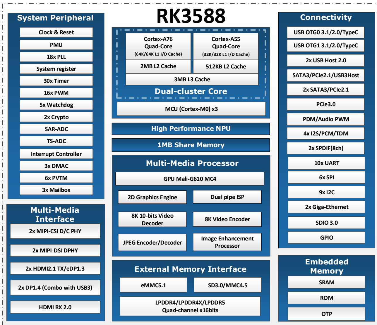
Fig. 1-1 Block Diagram
